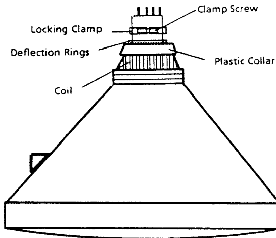
Figure 7.4 Yoke alignment
