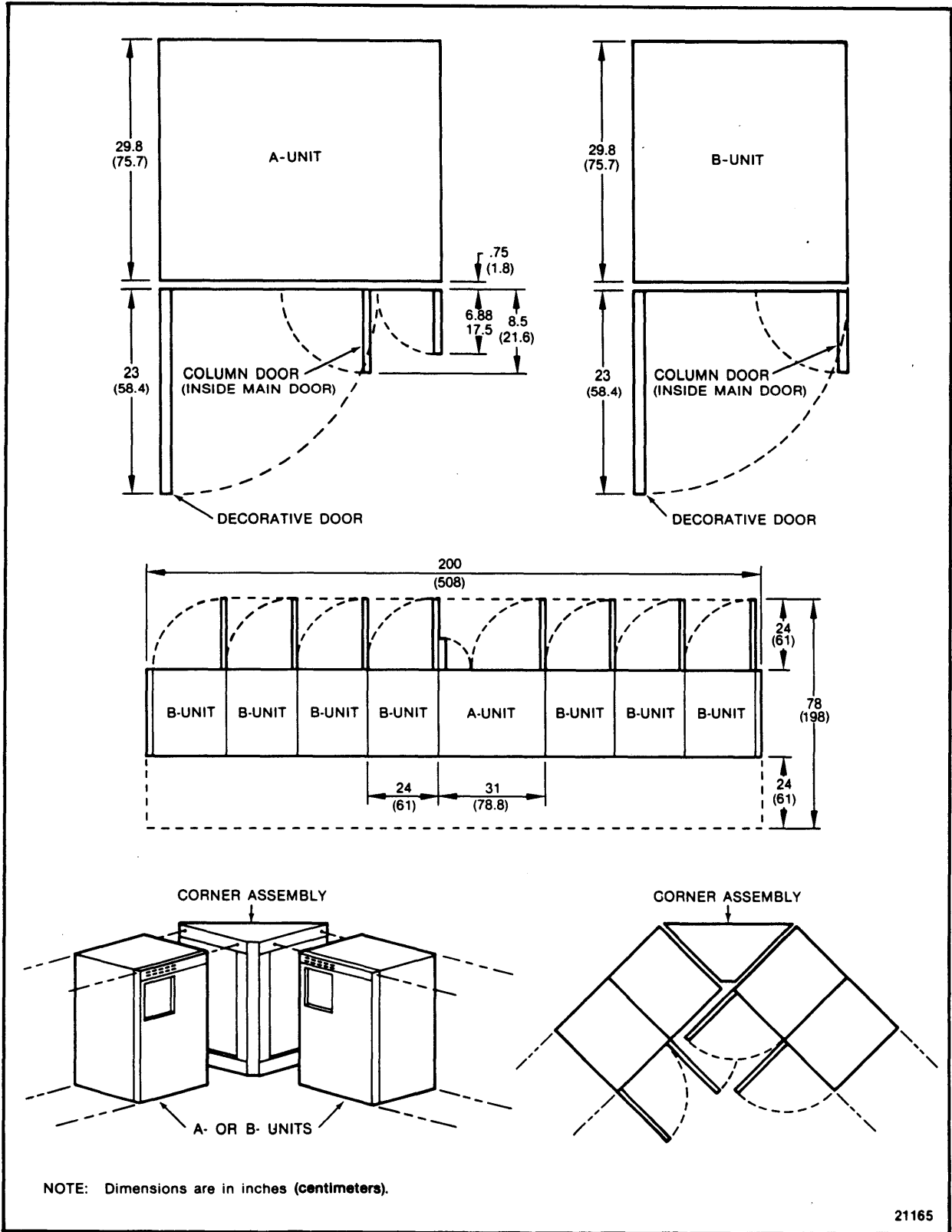
Figure 6-1. Floorspace Requirements
