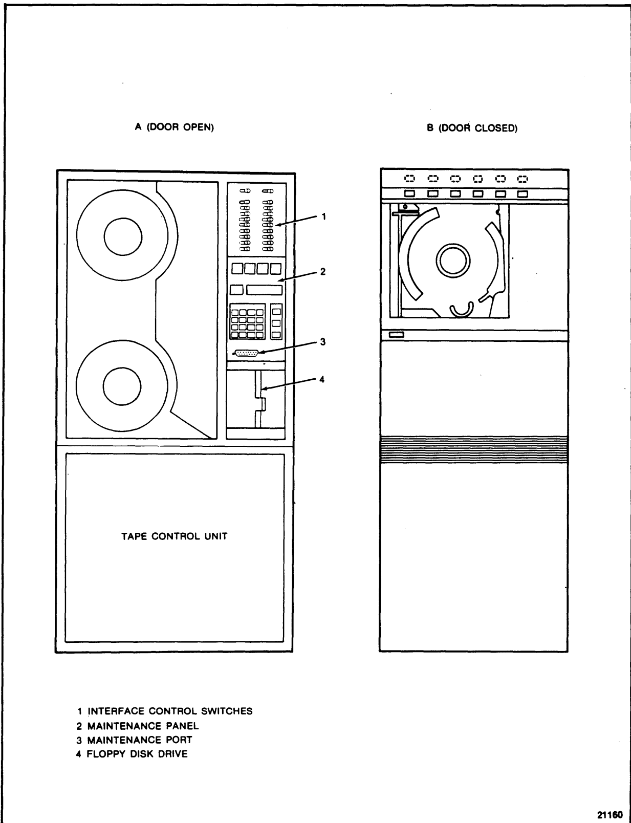
Figure 1-2. 4600 Tape Subsystem A- and B-Units
