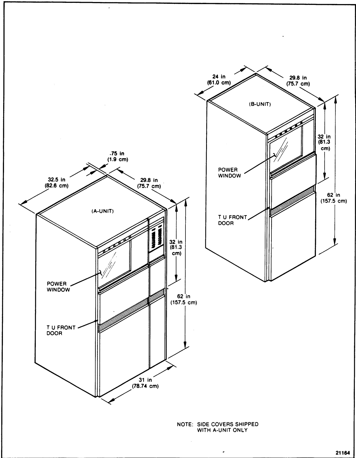
Figure 2-1. Tape Subsystem Dimensions
