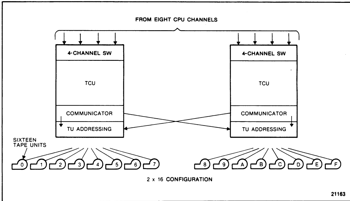
Figure 1-4. 2x16 Configuration
